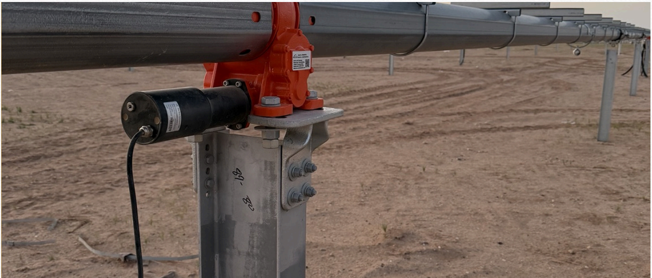
PV structure connection details
